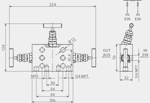
Three way valve group
