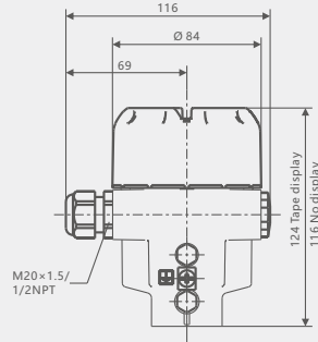
Single chamber housing, aluminum
