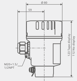
Single chamber housing, stainless steel, deep drawn
