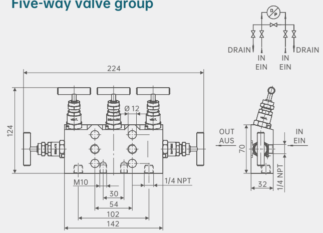
Five-way valve group
