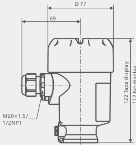
Single chamber housing, plastic
