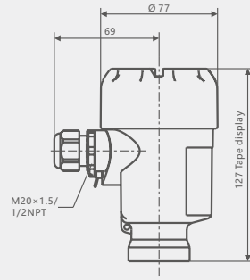
Single chamber housing, forged stainless steel
