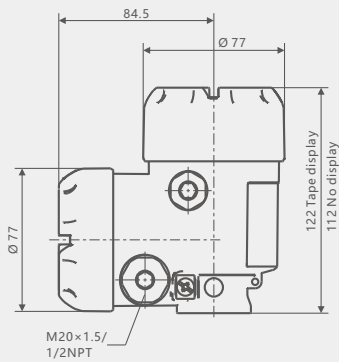
Double chamber housing, plastic
