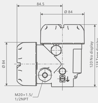
Double chamber housing, aluminum
