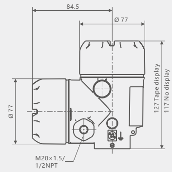
Double chamber housing, forged stainless steel
