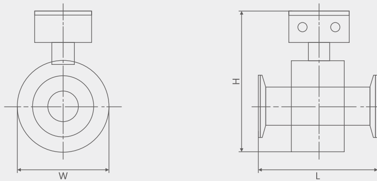
Fig. 7 Outline drawing of sanitary electromagnetic flow sensor
