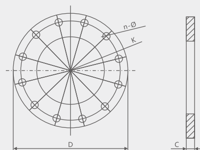
Figure 5 Connection flange diagram
