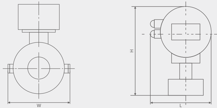
Fig. 6 Outline drawing of clamping electromagnetic flow sensor
